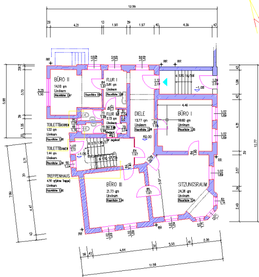
Ground Plan
